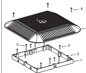
Fits most brands' existing 12" mud frames. Retrofits over all sumps/frames up to 15" using brass anchor kit
