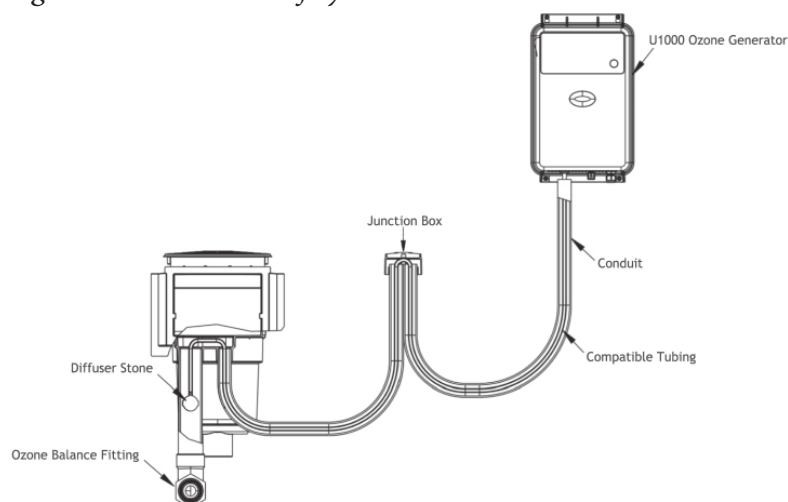
Figure 2.2 Front View of System
