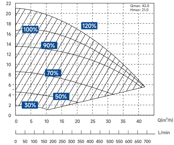
H(m) IP40
