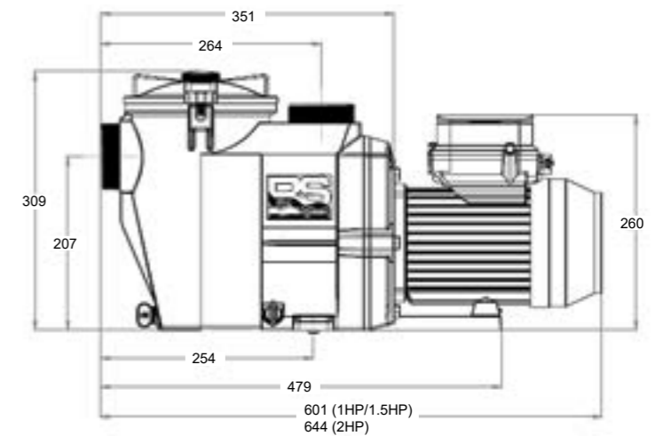
All dimensions in millimeters
