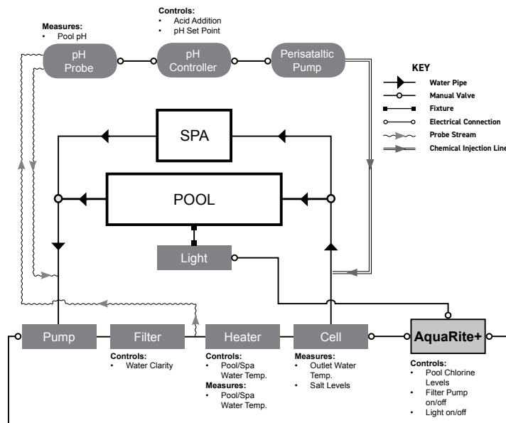
AquaRite+ as a Stand Alone Chlorinator
