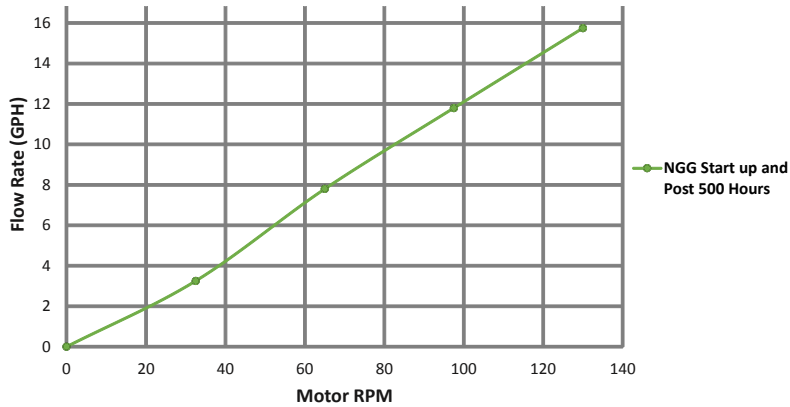
A2A NGG Output at various RPM
