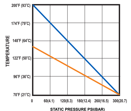
Maximum Temperature vs. Pressure
