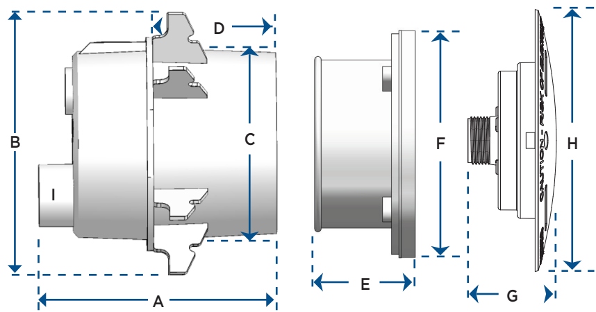
Spectrum™ 360 Flush Mounted Pool Light - Gunite
