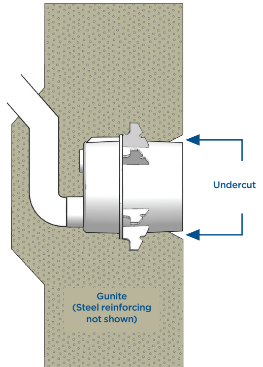
Diagram 1 – After Guniting/Shotcreting
