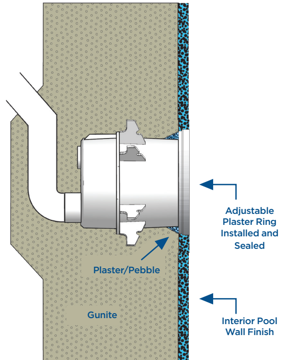
Diagram 3 - Sealing
