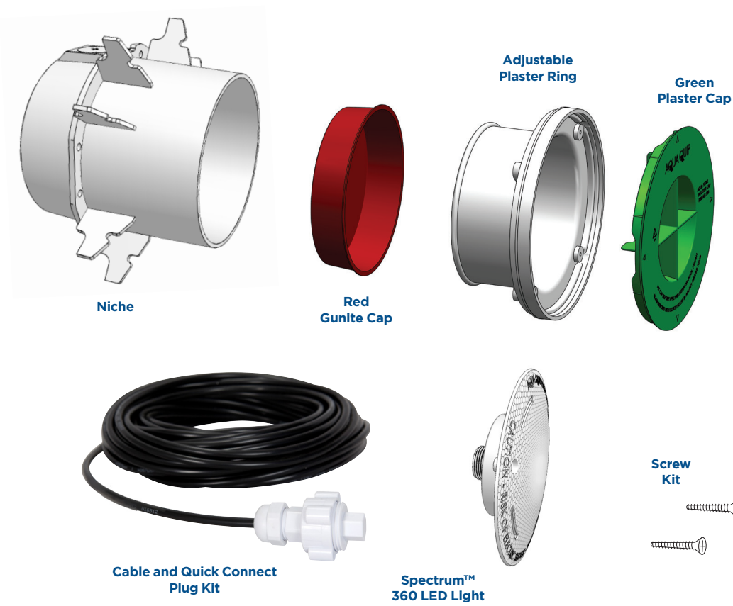
Spectrum™ 360 Flush Mounted Pool Light - Gunite
