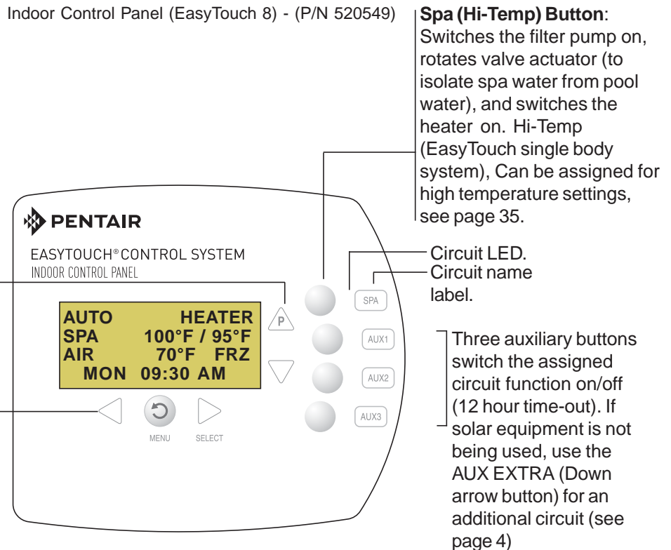
Indoor Control Panel (EasyTouch 4) - (P/N 520548)
