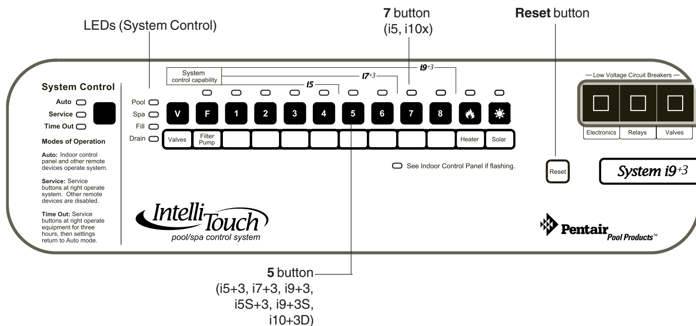
Main Outdoor Control Panel (Located in the Load Center or Power Center)
