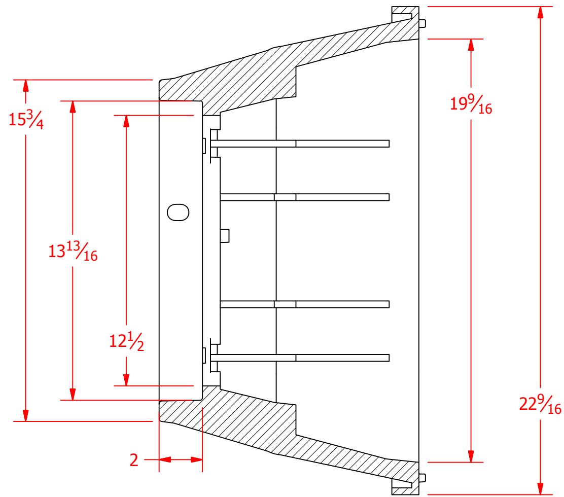
SECTION A-A (COVER REMOVED)
