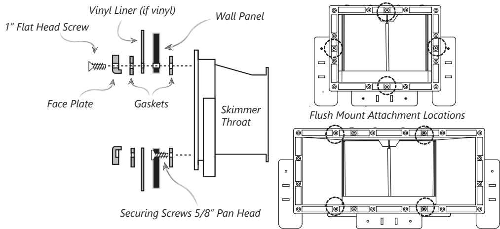
FIGURE 3: FLUSH-MOUNT INSTALLATION
