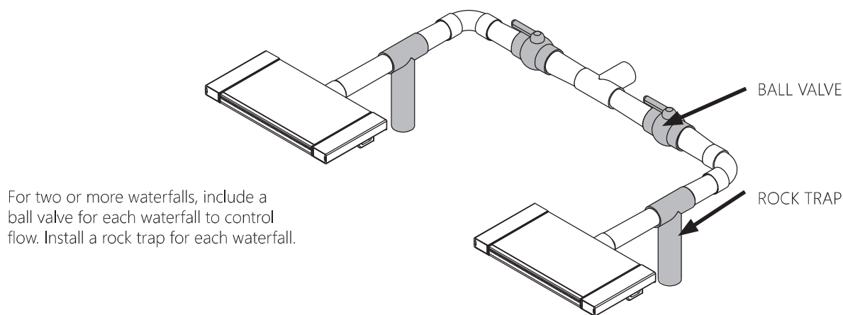
Figure 10: Multi-Waterfall Valving
