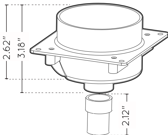
MULTI-NOZZLE DECK JET SIDE VIEW
