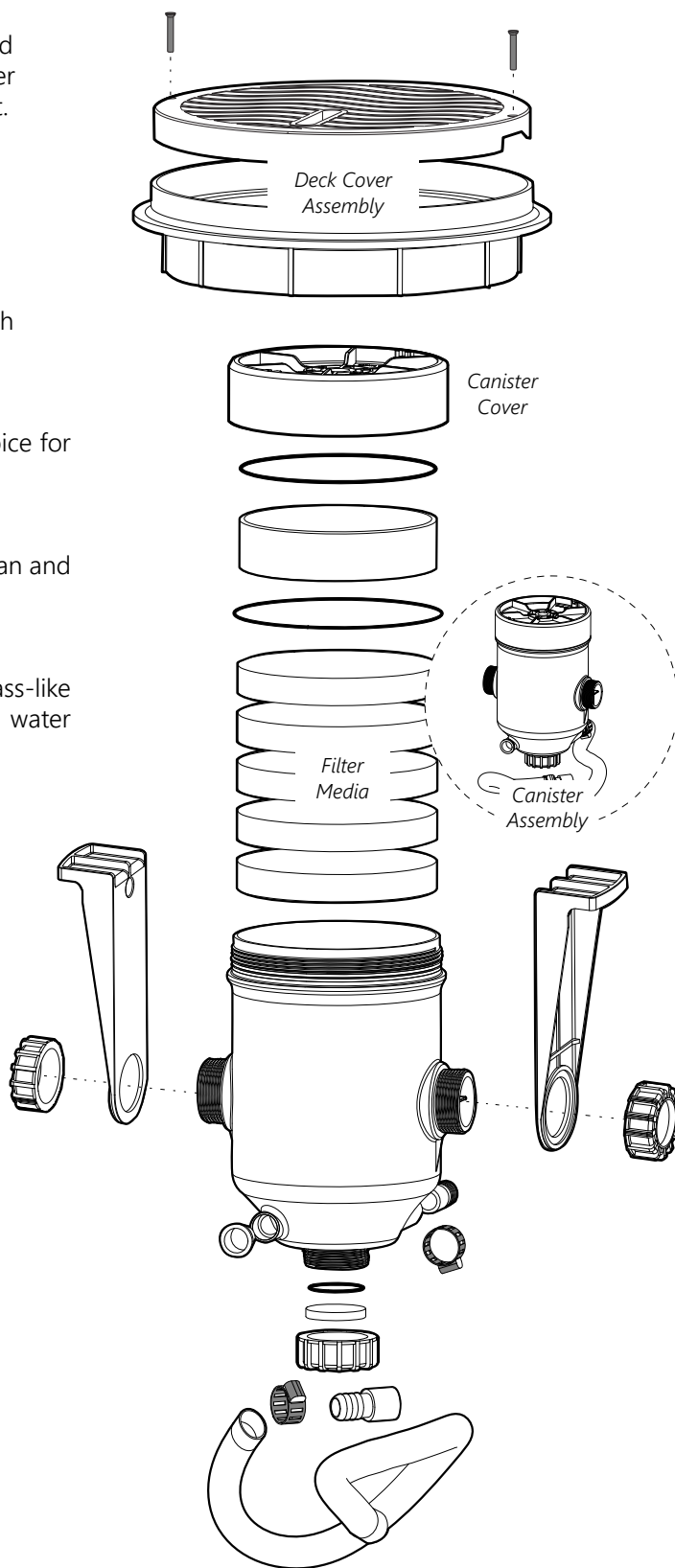
EXPLODED COMPONENT VIEW
