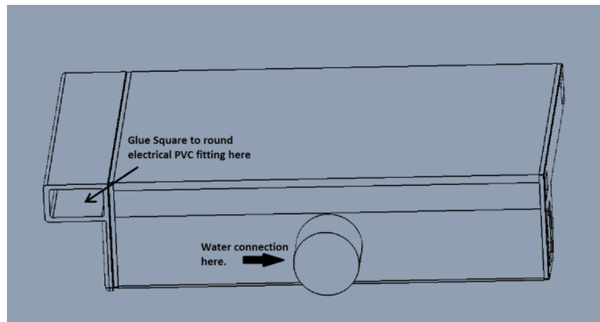
Figure 5: PVC Conduit on both ends
