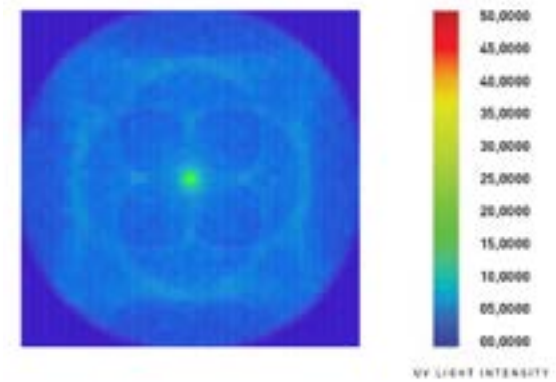
Stainless steel radiation pattern 7.5cm from end cap
