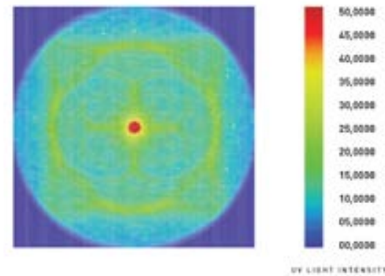
Electro special casing radiation pattern 7.5cm from end cap
