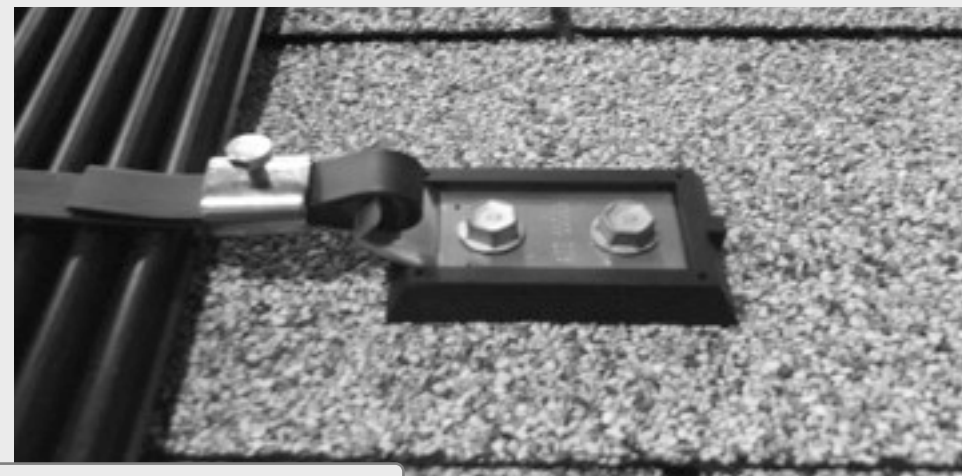
FIGURE 8 Termination Strap Bracket Assembly
