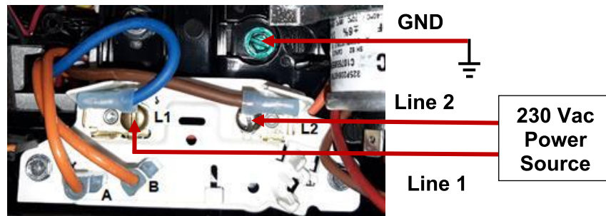
AC Terminal Block Wiring for 230 Vac
