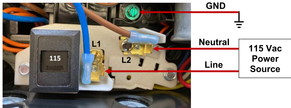
AC Terminal Block Wiring for 115 Vac
