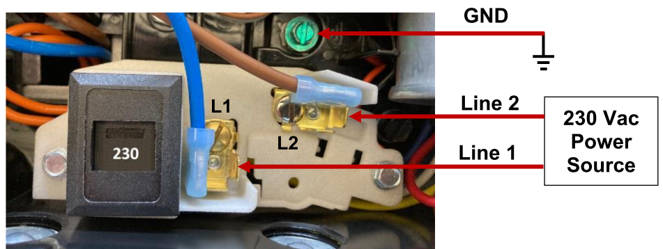
AC Terminal Block Wiring for 230 Vac
