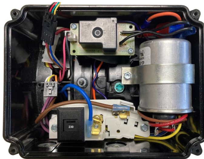
Wiring Compartment
