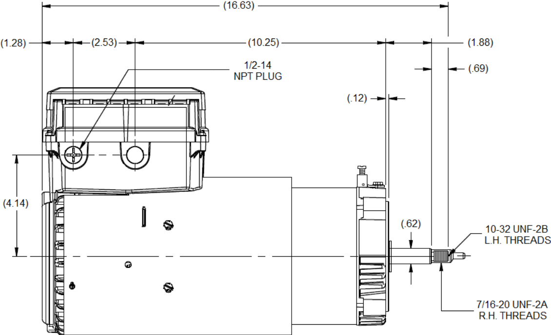
Side View
