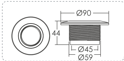
Suction Fitting
