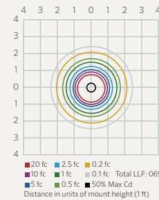
RW 6LED ISOFOOTCANDLE PLOT
