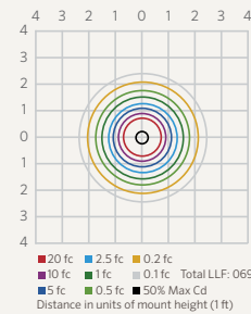
RW 3LED ISOFOOTCANDLE PLOT
