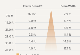
RW 9LED ILLUMINANCE AT A DISTANCE
