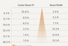
RW 6LED ILLUMINANCE AT A DISTANCE
