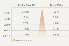
RW 1LED ILLUMINANCE AT A DISTANCE
