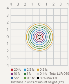
RW 1LED ISOFOOTCANDLE PLOT
