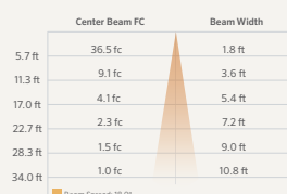
RW 3LED ILLUMINANCE AT A DISTANCE
