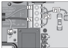
1-phase L1 current returns through neutral Connect PJ1 between P7 and P13. Connect PJ2 between P10 and P74.
