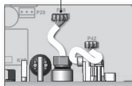
Regulation probe
