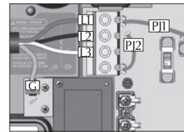
2-phase used from 3-phase Delta — no neutral Use 2-phase setting L1+L2 currents return through L3 Connect PJ1 between P7 and P10. Connect PJ2 between P13 and P74.
