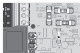
Transformer fuse
