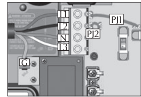
3-phase with single neutral L1, L2+L3 currents return through neutral Connect PJ1 between P7 and P10. Connect PJ2 between P11 and P13.
