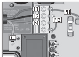
2-phase with single neutral L1+L2 currents return through neutral Connect PJ1 between P7 and P10. Connect PJ2 between P13 and P74.
