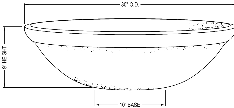
PERSPECTIVE
