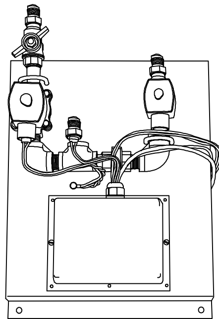
SUB PANEL
