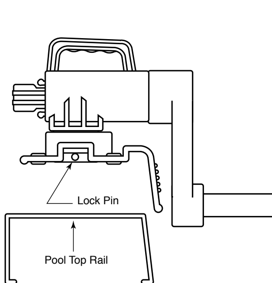
NON-PERMANENT ASSEMBLY
