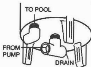
FIG 1: Betterfilter® Models BF42, BF84, BF126
