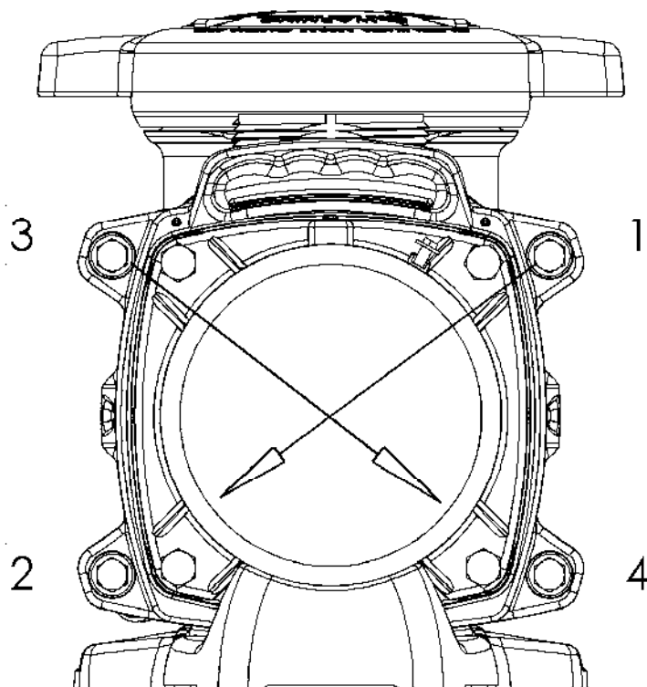
HOUSING BOLT TORQUE PATTERN
