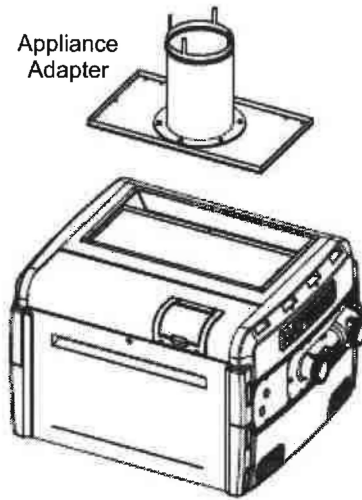
Figure5 Adapter Install
