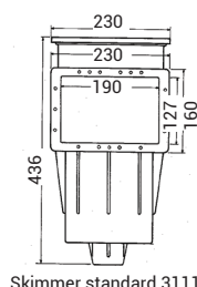
Skimmer standard 3111
