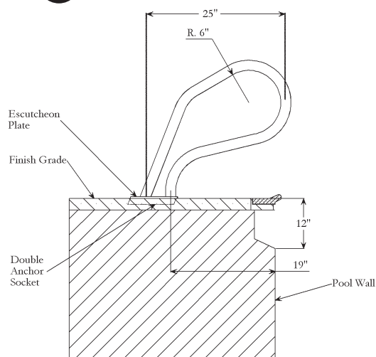
SECTION
