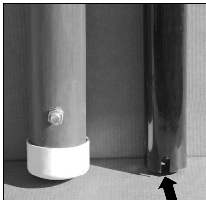
Anchor and Support Pole ... Notches in Pole Align Notches with Bolt or Rod in Anchor
