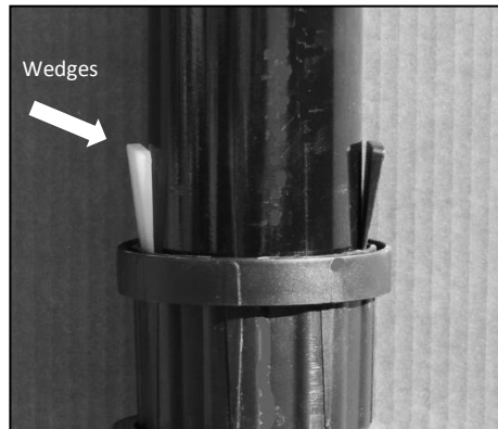
Wedges Between Pole Adapter and Support Pole
