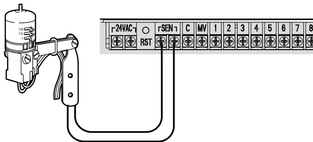
Mini-Clik Rain Sensor
