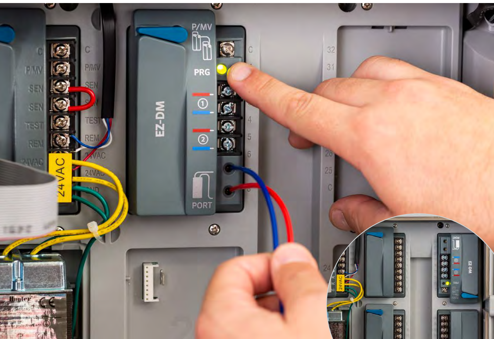
Hybrid Installation
