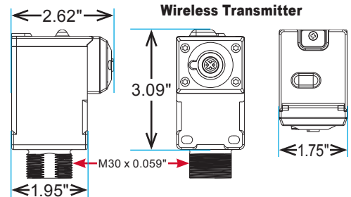
Wireless Transmitter
