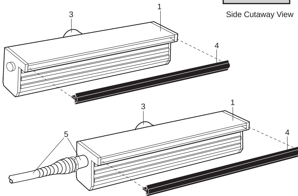
Figure 2. Sheer Descent and FiberFall Components
