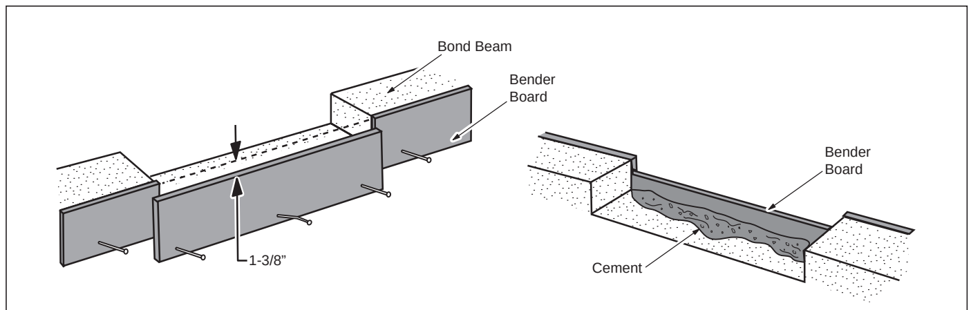
Figure 5. Install Bender Board
