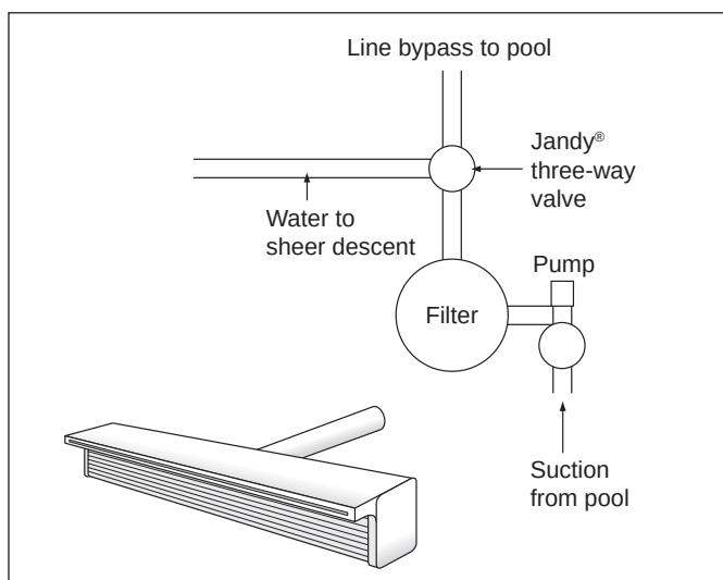
Figure 13. Three-Way Valve Plumbing Setup
