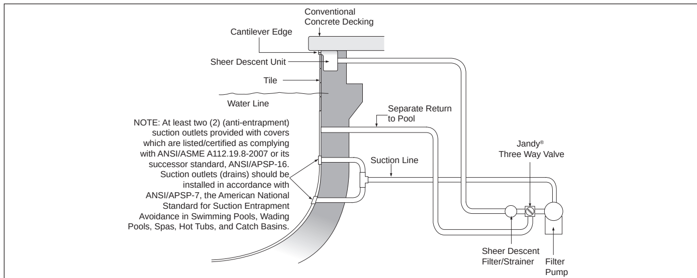
Figure 12. Filter Pump Installation
