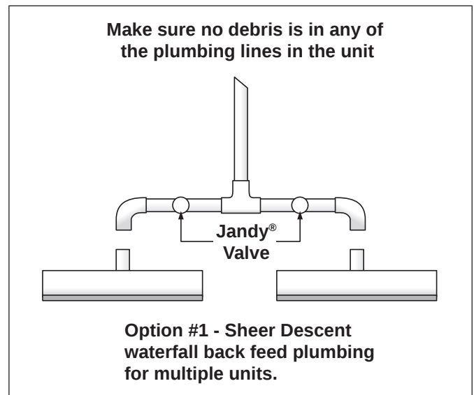
Figure 15. Multiple Sheer Descent Plumbing Setup
