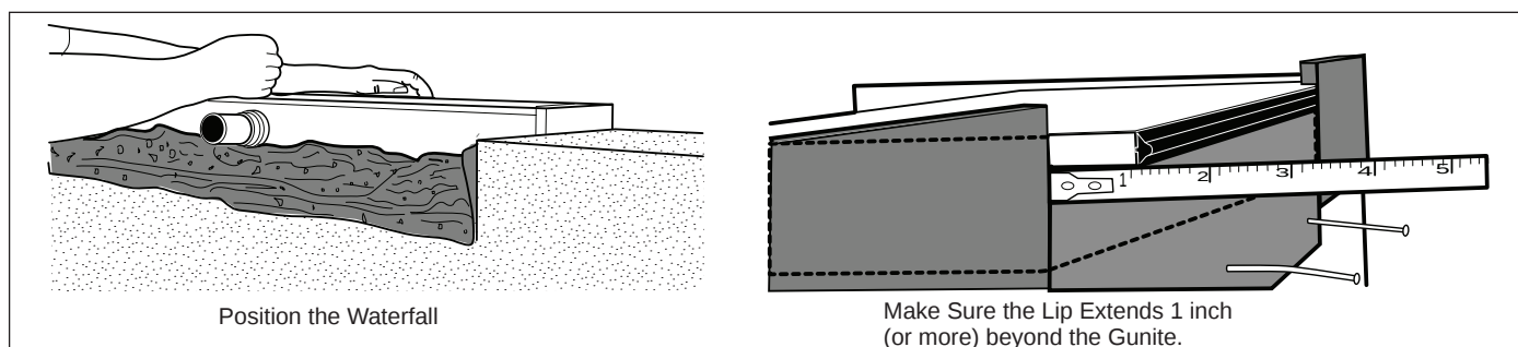
Figure 7. Positioning the Waterfall in Notch
