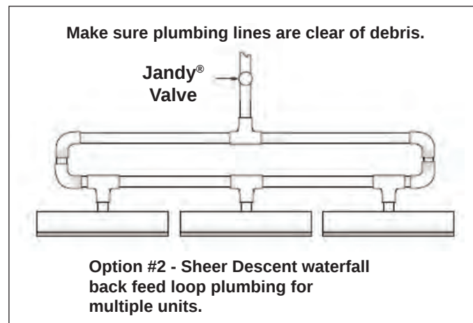
Figure 16. Multiple Sheer Descent Loop Plumbing Setup
