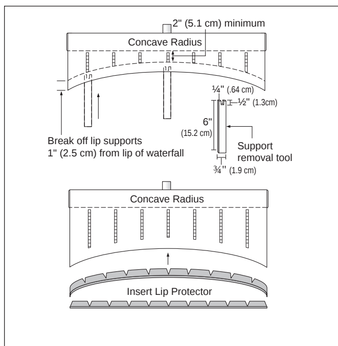
Figure 18. Custom Installations - Concave Radius
