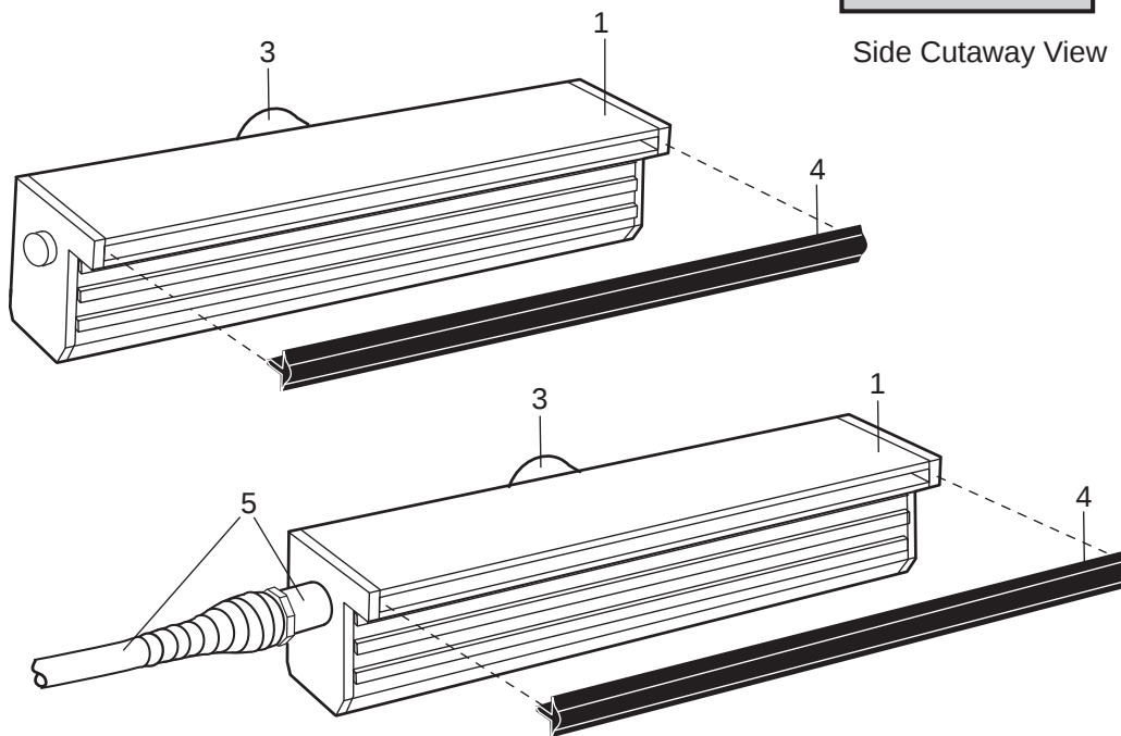
Figure 2. Sheer Descent and FiberFall Components
