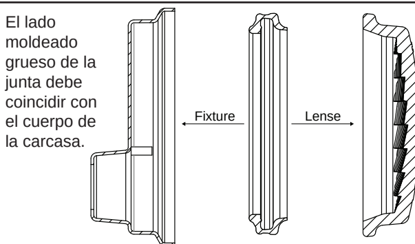
Figura 10. Corte transversal de la luz LED blanca Jandy Pro Series
