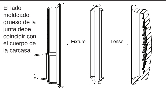
Figura 10. Corte transversal de la luz LED blanca Jandy Pro Series
