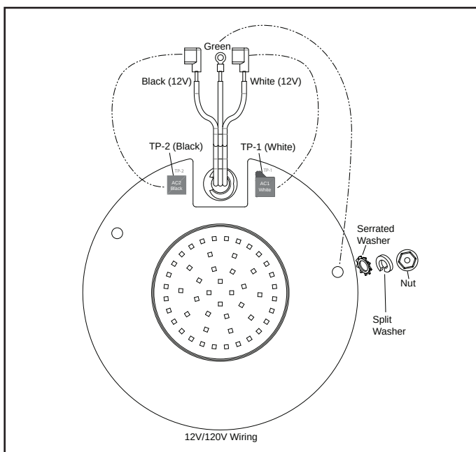
Figure 8. Large Light Engine (PCB) Replacement and Wiring
