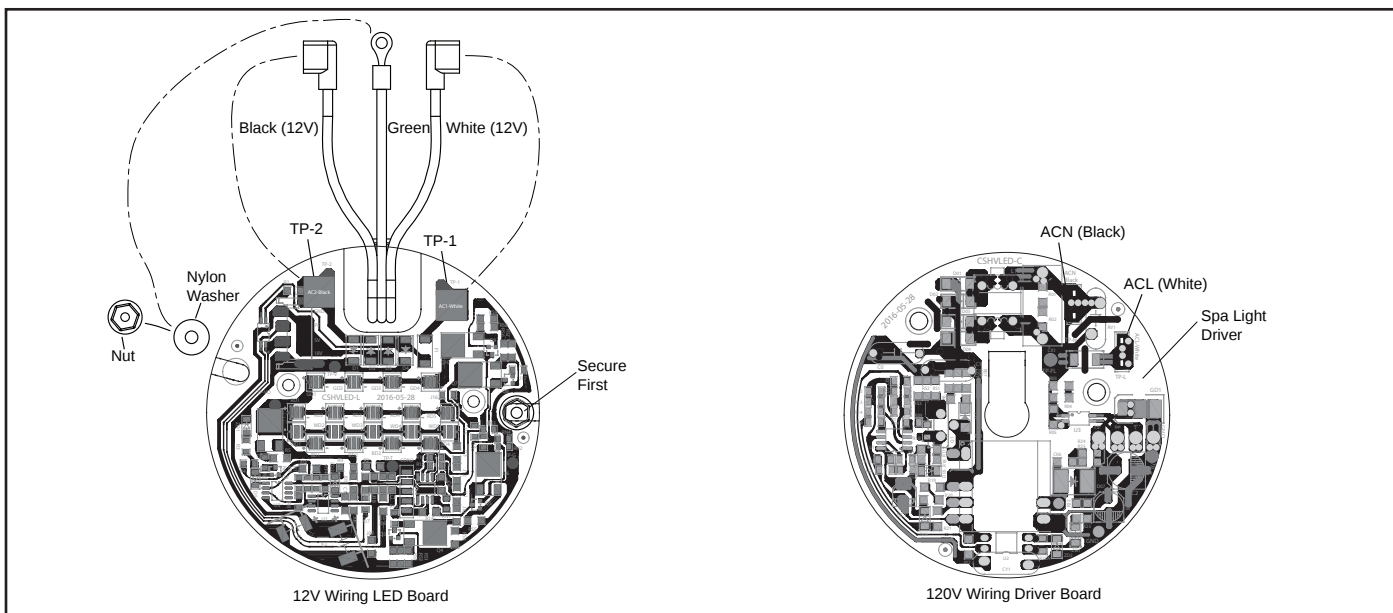
Figure 7. Small Light Engine (PCB) Replacement and Wiring
