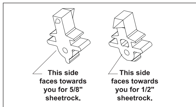
Figure 30. Cleat Orientation
