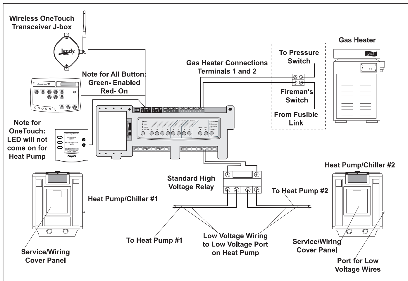
Figure 19. Heater and Heat Pump/Chiller Wiring
