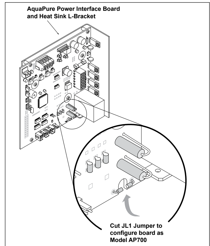
Figure 9. AquaPure® Power Interface Board
