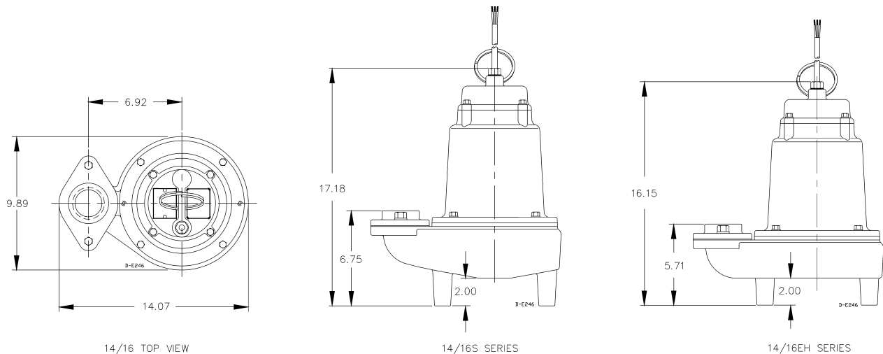
Figure 1 - Dimensions
