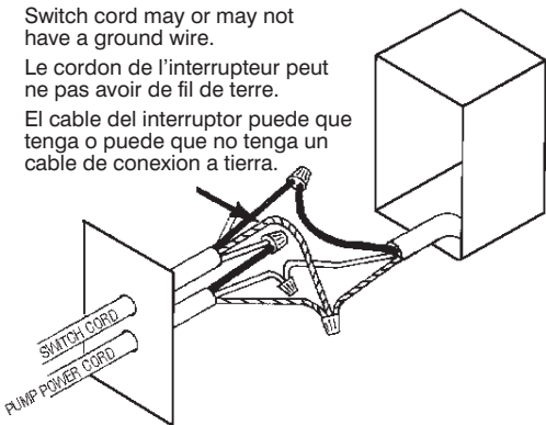
Figure 5 Installation Instalacion 230V
