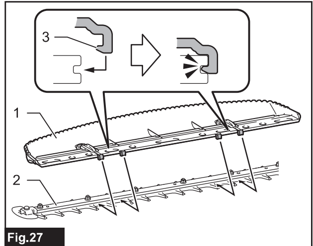
► 1. Chip receiver 2. Shear blades 3. Claw
