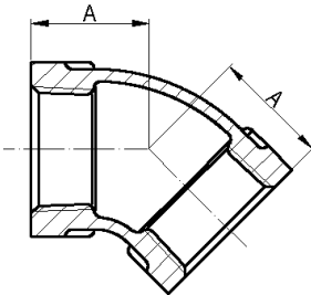
Brass Elbow 45
