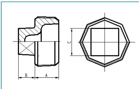
Brass Plug
