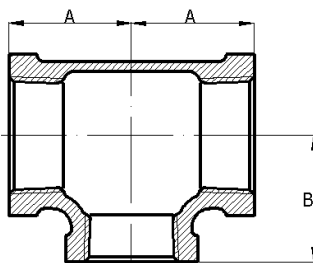
Brass Reducing Tee
