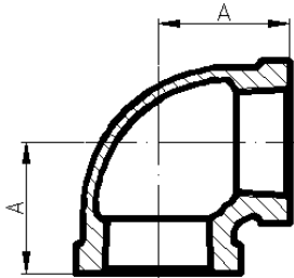
Brass Elbow 90
