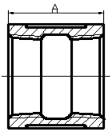
Brass Coupling
