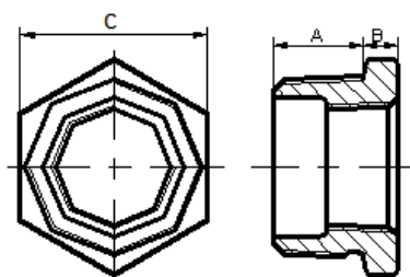
Brass Bushing
