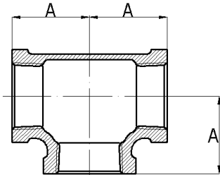
Brass Tee
