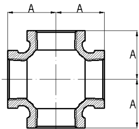
Brass Cross
