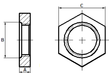
Brass Locknut
