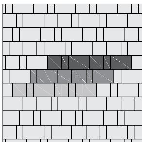
3-PIECE RUNNING BOND PATTERN
