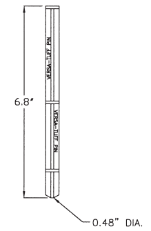
VERSA-TUFF PIN PIN DIMENSIONS SCALE: NONE
