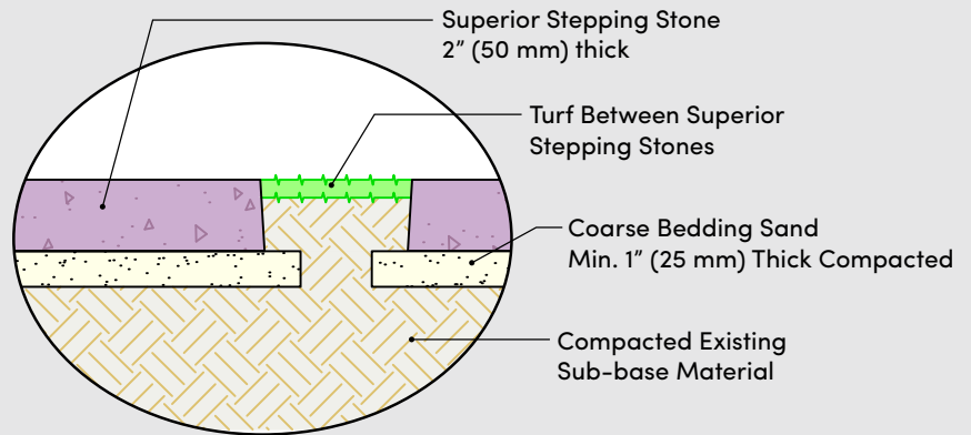
Typical Cross-Section
