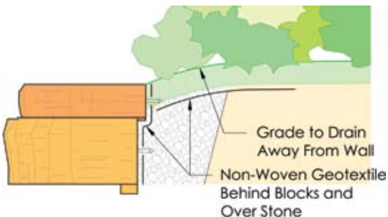
Plant appropriate vegetation on the back of the wall
